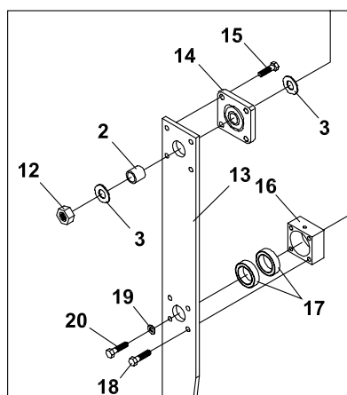
18" / 24" CUTTING HEAD
