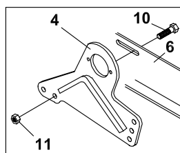
16" / 18" CUTTING HEAD
