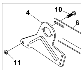
24" CUTTING HEAD
