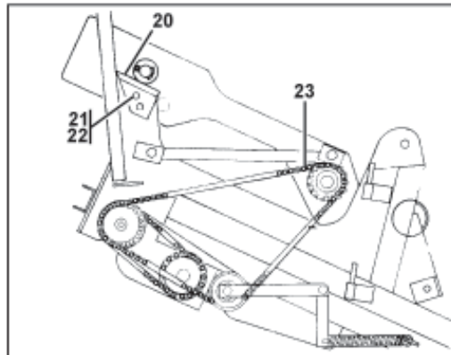
COMP. ROLL-UP CONVEYOR FIGURE 52 SOD HARVESTER
