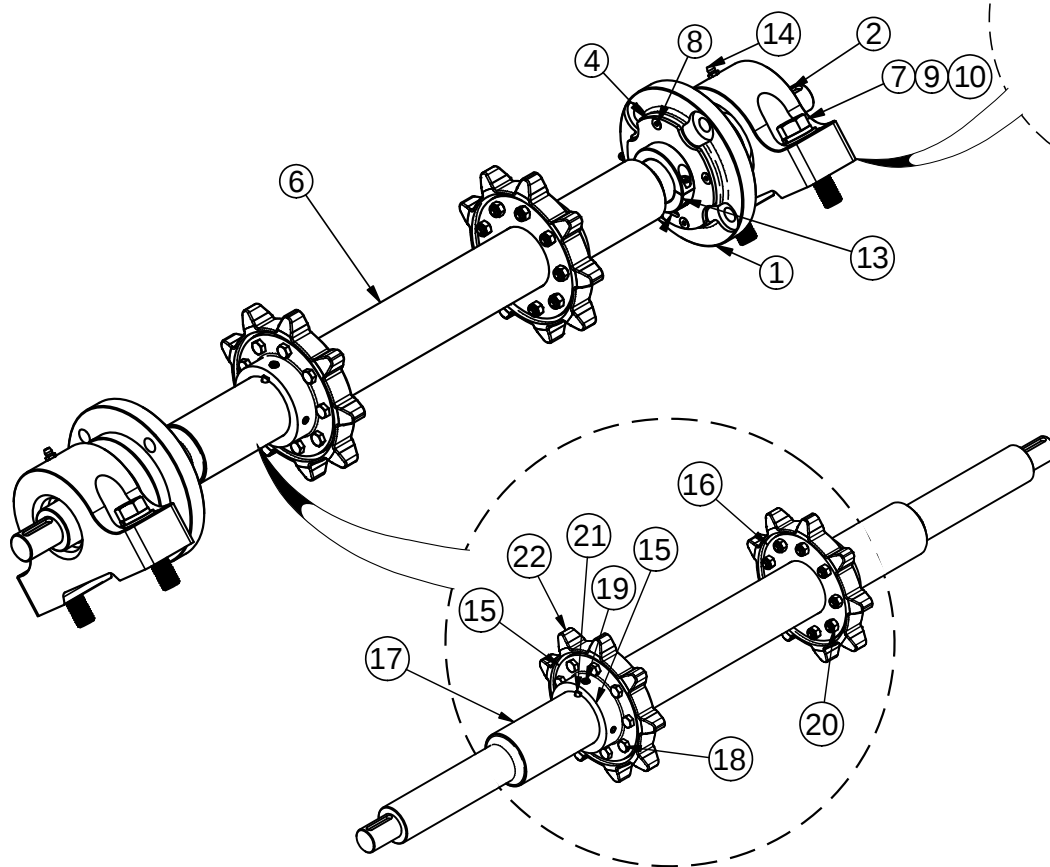
Conveyor Drive Shaft Assembly - 1.50 Shaft
