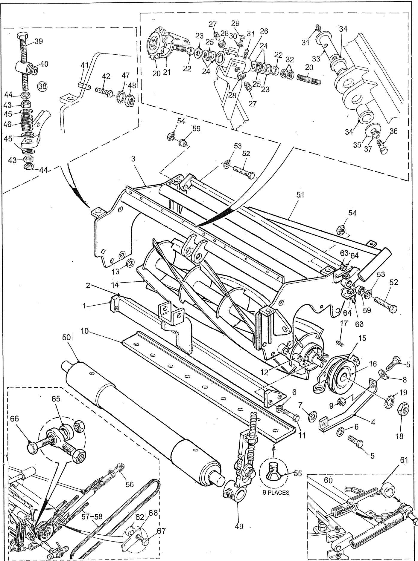
FAIRWAY MOWER REEL ASSEMBLY (TYPICAL)
