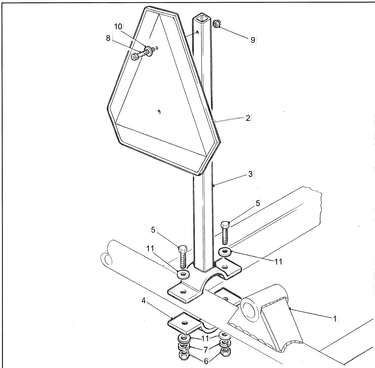
SLOW MOVING VEHICLE EMBLEM (OPTION)
