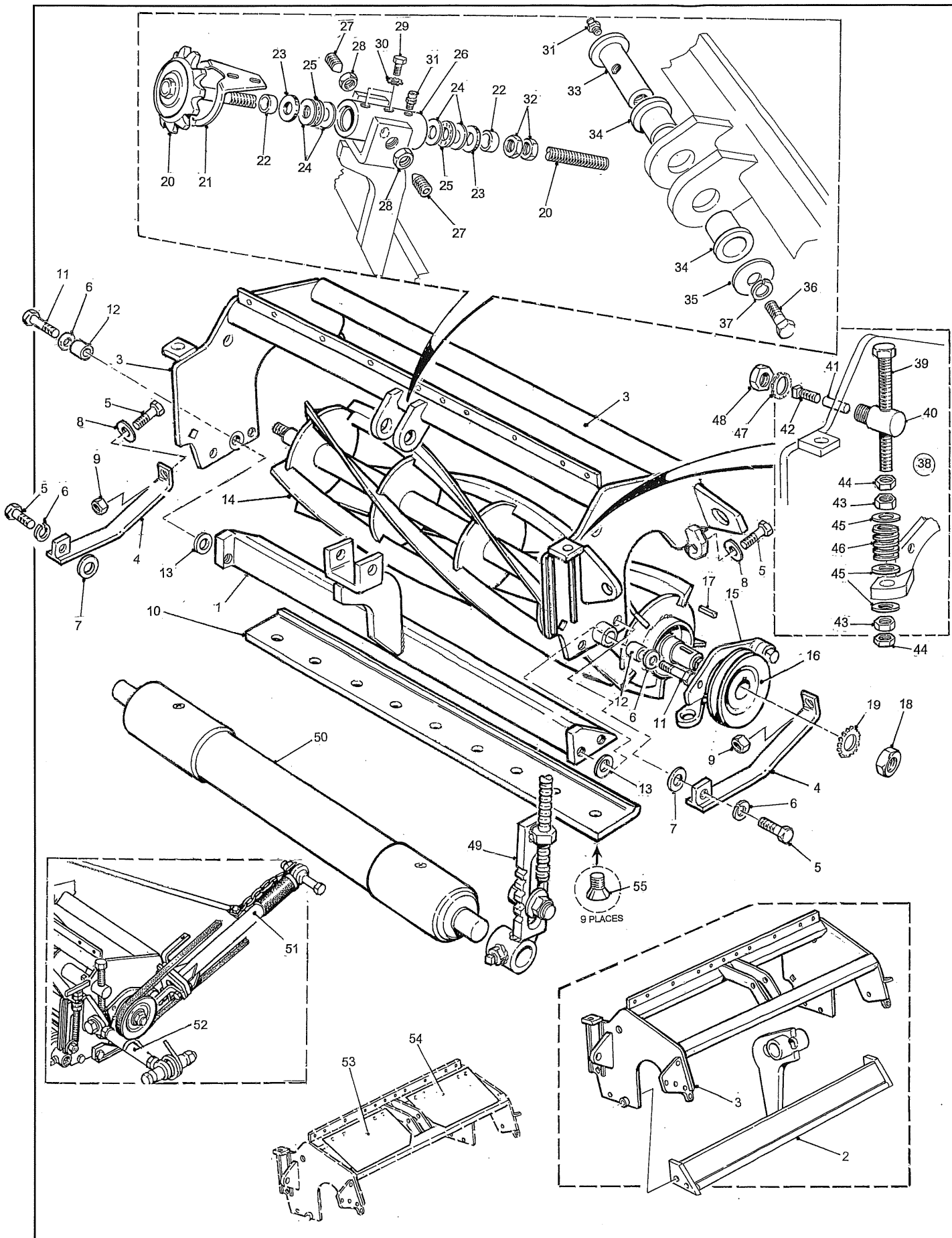
SINGLE POINT ADJUSTMENT REEL ASSEMBLY (OPTION)
