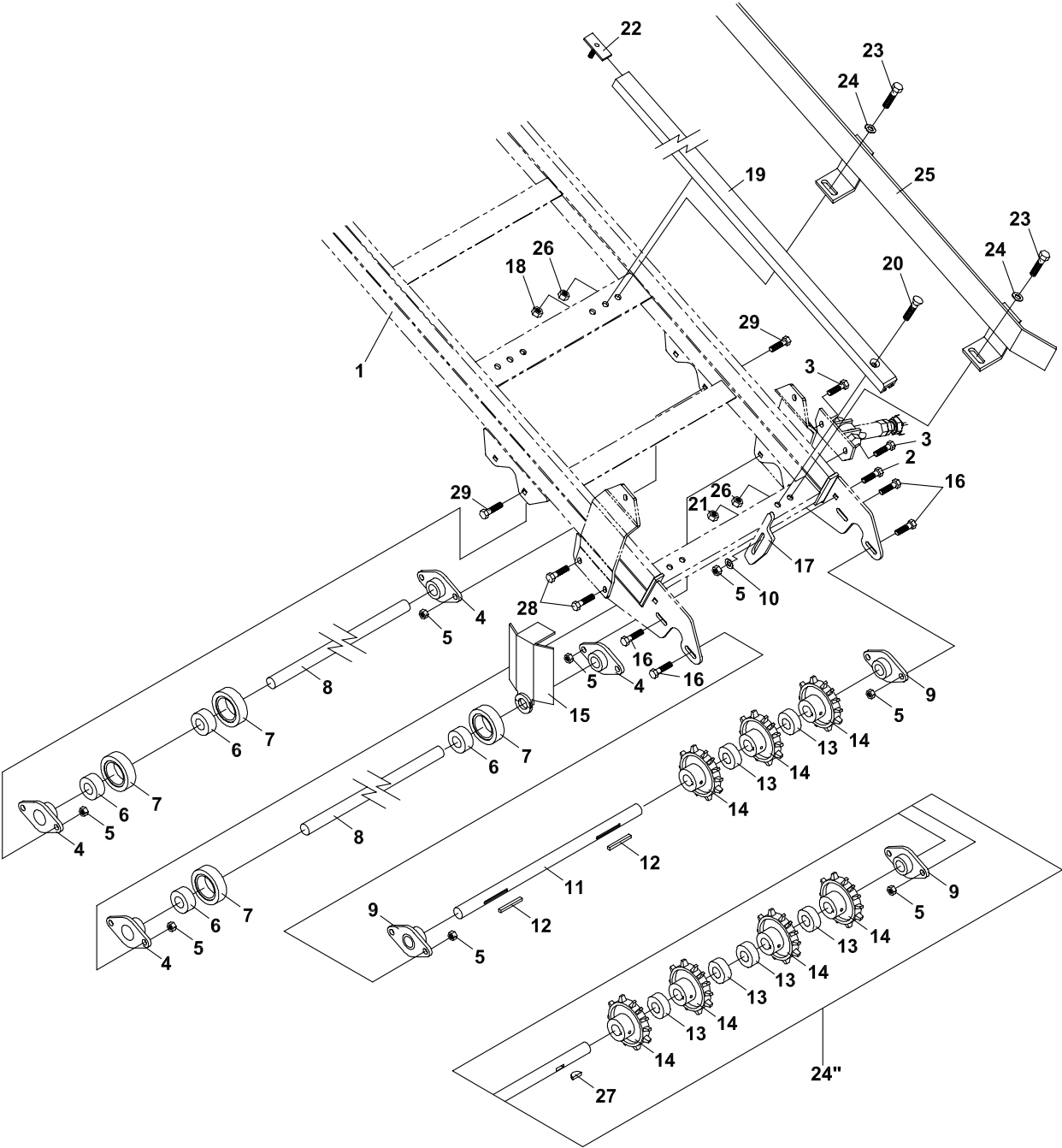
FRONT IDLERS & SLIDERS MINTEX MAT - 16", 18" & 24"
