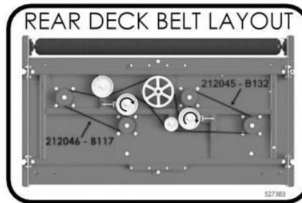
527383 REAR DECK BELT LAYOUT
