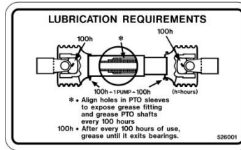
526001 100HR DECAL – PTO GREASE
