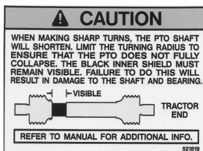
521819 DECAL – CAUTION
