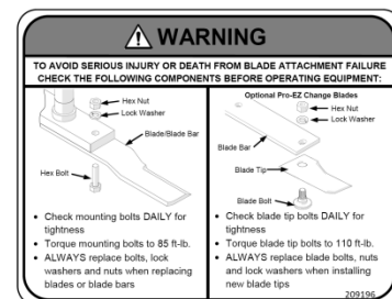
209196 DECAL – BLADE HARDWARE
