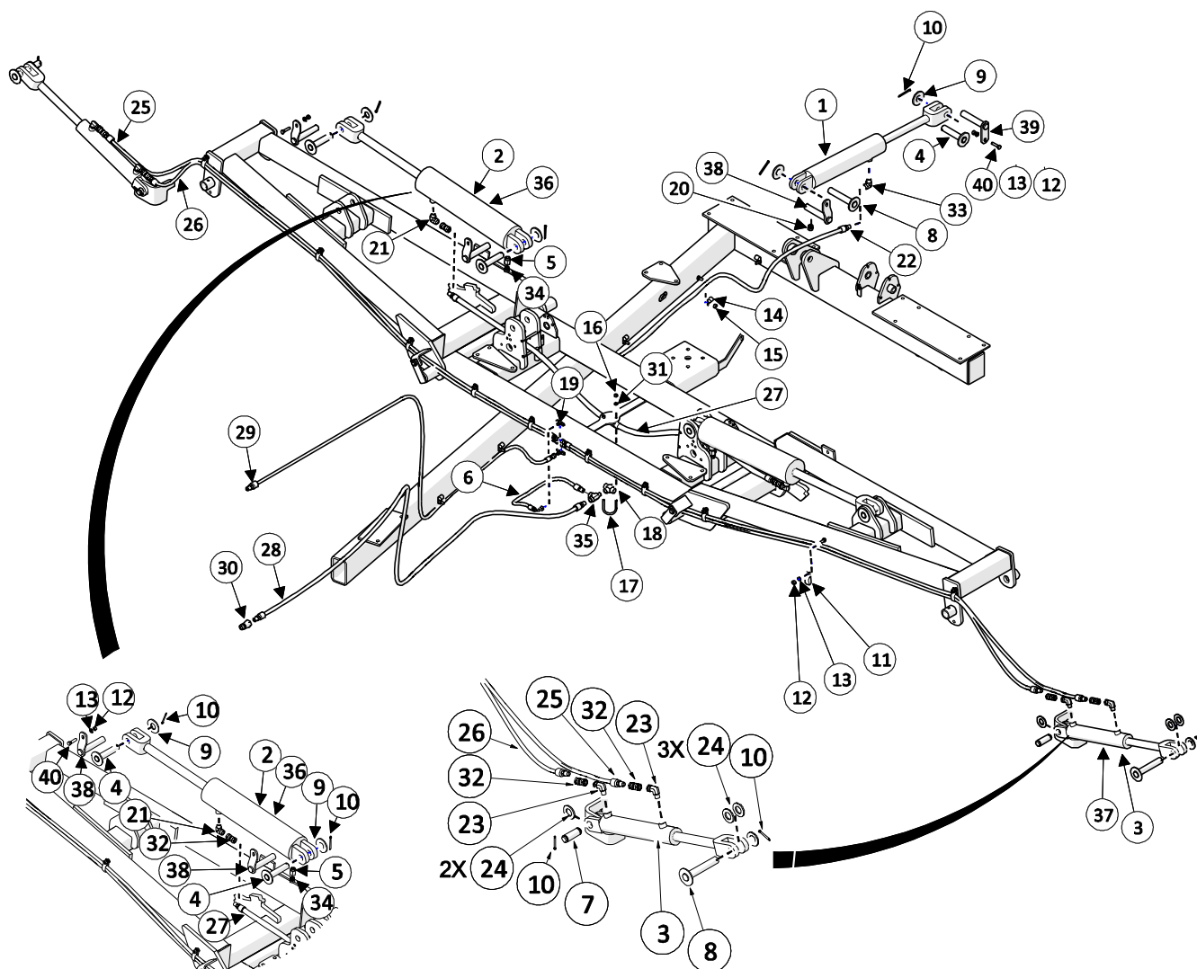
MAIN WING CYLINDERS
