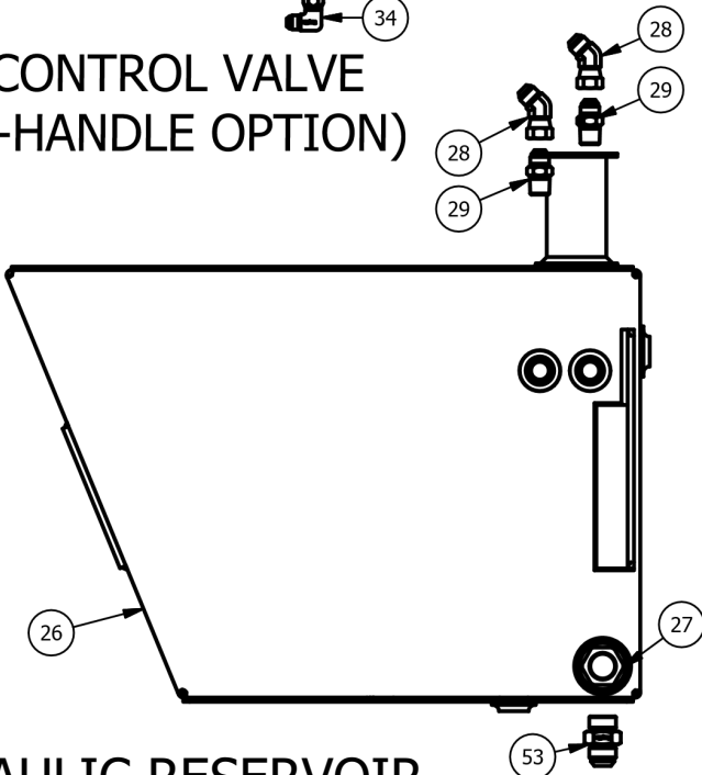
HYDRAULIC RESERVOIR
