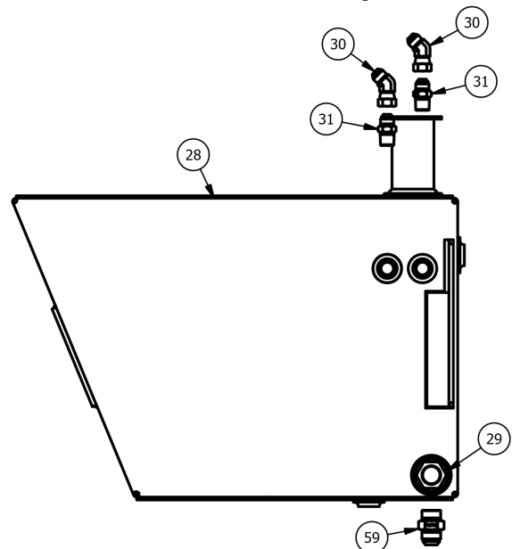
HYDRAULIC RESERVOIR
