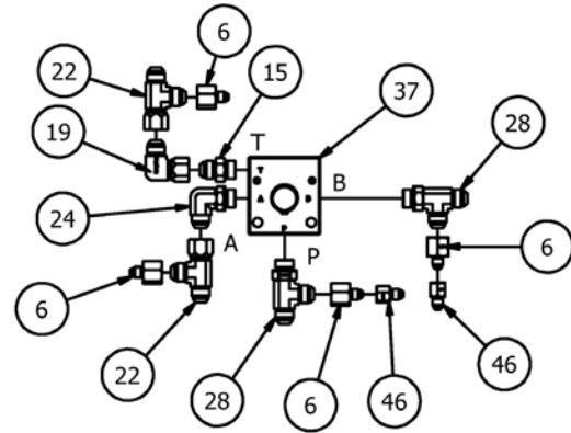
2WD/4WD/INBOARD VALVE "B"
