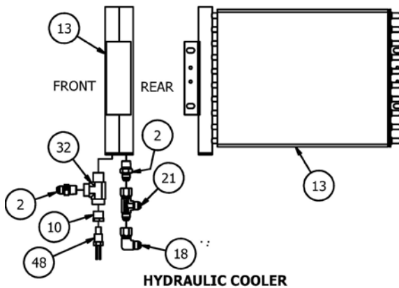
HYDRAULIC COOLER
