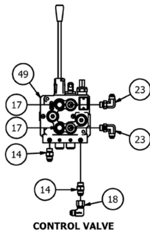
CONTROL VALVE
