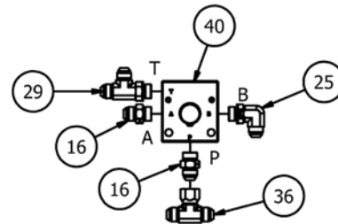
2WD/4WD/INBOARD VALVE "A"
