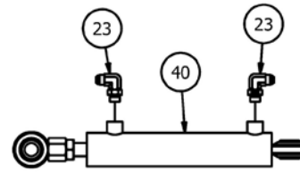
STEERING CYLINDER
