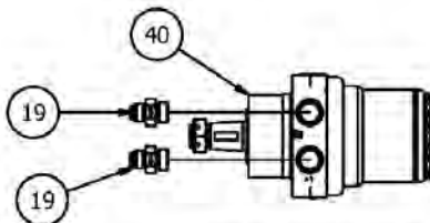
LEFT FRONT MOTOR
