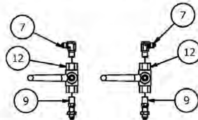
FRONT WHEEL LOCK VALVES
