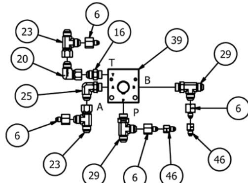
2WD/4WD/INBOARD VALVE "B"
