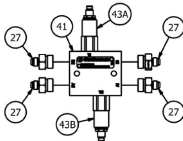
STEERING RELIEF
