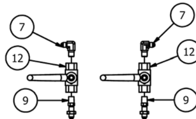
FRONT WHEEL LOCK VALVES
