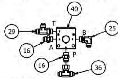
2WD/4WD/INBOARD VALVE "A"
