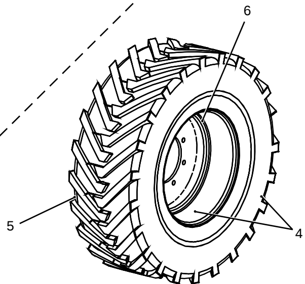
OPTIONAL FRONT WHEEL ASSEMBLY
