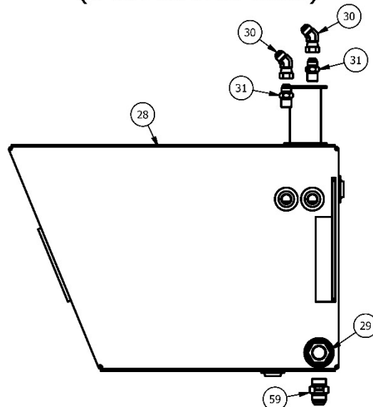
HYDRAULIC RESERVOIR
