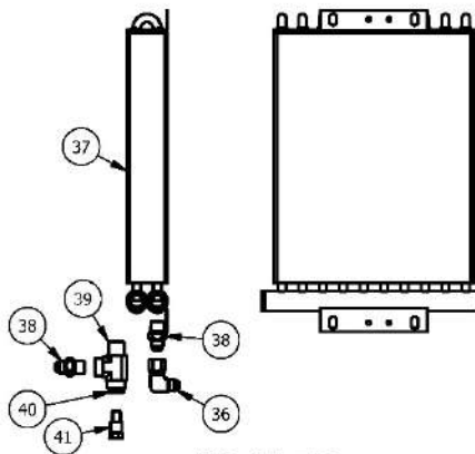
COOLER
