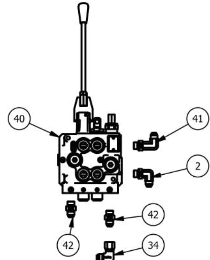
CONTROL VALVE (NON T-HANDLE)
