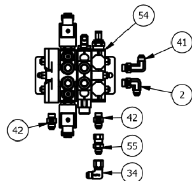
CONTROL VALVE (T-HANDLE OPTION)
