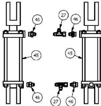
LIFT CYLINDERS
