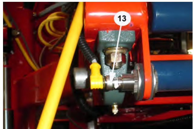
13. Push Bar 'Home'. Sensor to Target 1/8in. to 1/4in. Part No. KE10155 – 8 MM Inductive Proximity Switch
