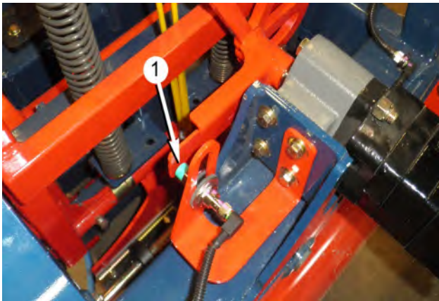
1. Cut-Off - Sensor to Target 1/4 in. to 3/8 in. Part No. KE10174 – 15 MM Inductive Proximity Switch
