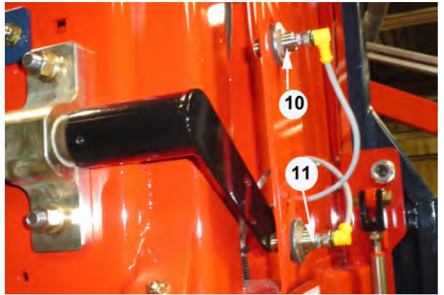
10/11. Paddles 'Up-Down' Sensor to Target 1/8in. to 1/4in. Part No. KE10155 – 8 MM Inductive Proximity Switch
