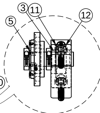
Conveyor Drive Shaft Assembly - 1.50 Shaft
