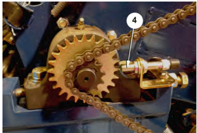
4. Roll Flap (Tooth Count) Sensor to Target 1/8 in.max Part No. KH30088 - Conveyor Motor with High Speed Sensor – CURRENT Part No. KH30089 – High Speed Sensor – CURRENT Part No. 4132981 – 4 MM Inductive Sensor – N/C
