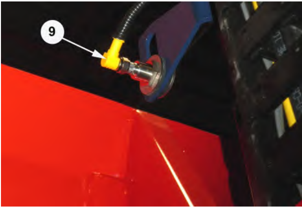
9. Pallet Disp'. 'High'. Sensor to Target 1/8in. to 1/4in. Part No. KE10155 – 8 MM Inductive Proximity Switch
