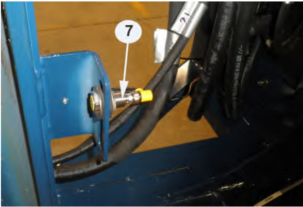
7. Pallet Disp'. 'Bottom'. Sensor to Target 1/8in. to 1/4in. Part No. KE10155 – 8 MM Inductive Proximity Switch
