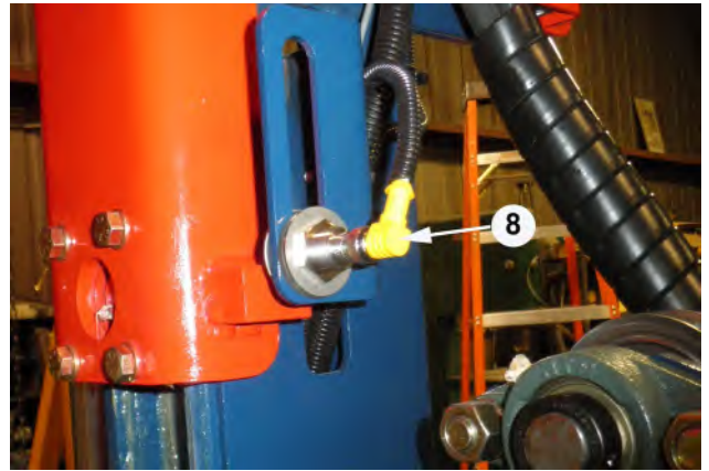
8. Pallet Disp'. 'Mid.' Sensor to Target 1/8in. to 1/4in. Part No. KE10155 – 8 MM Inductive Proximity Switch
