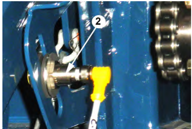
2. Conveyor 'DOWN' - Sensor to Target 1/8 in. to 1/4 in. Part No. KE10155 – 8 MM Inductive Proximity Switch
