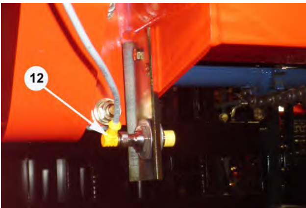
12. Push Bar 'Away' Sensor to Target 1/4in. to 3/8in. Part No. KE10155 – 8 MM Inductive Proximity Switch
