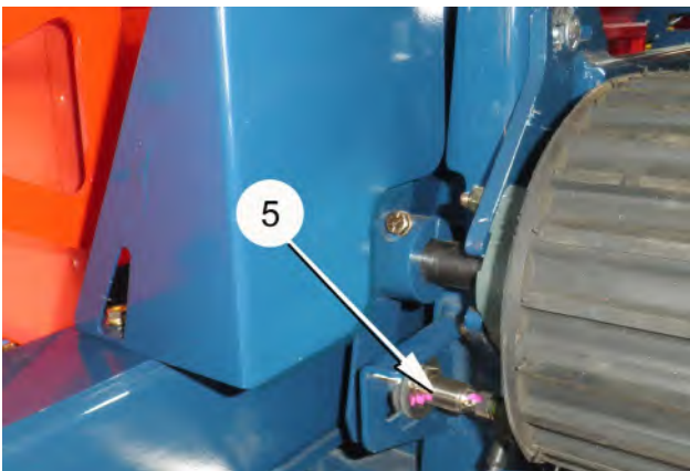
5. Index Conv'. 'CLEATS' position Sensor to Target . 1/8 in. to 1/4in Part No. KE10155 – 8 MM Inductive Proximity Switch
