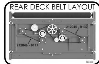
527383 REAR DECK BELT LAYOUT
