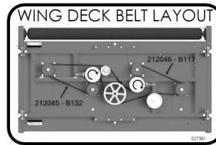
527381 WING DECK BELT LAYOUT
