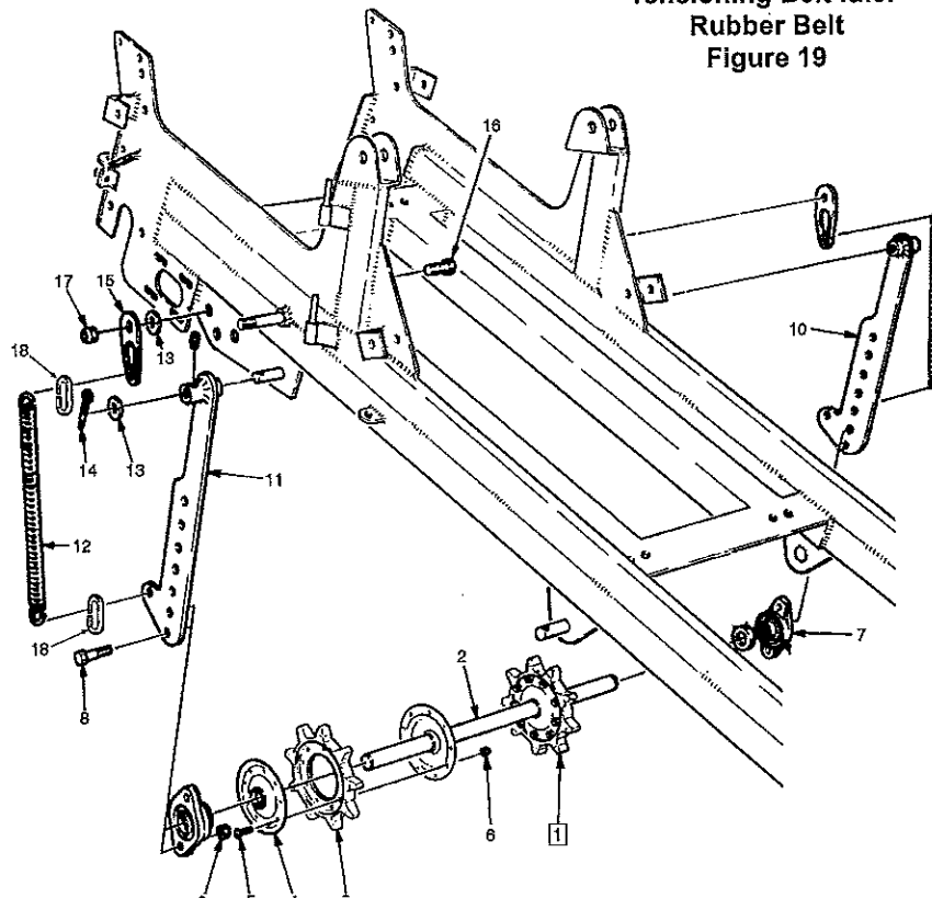
Motor Guard Assembly Mintex Belt Figure 19A
