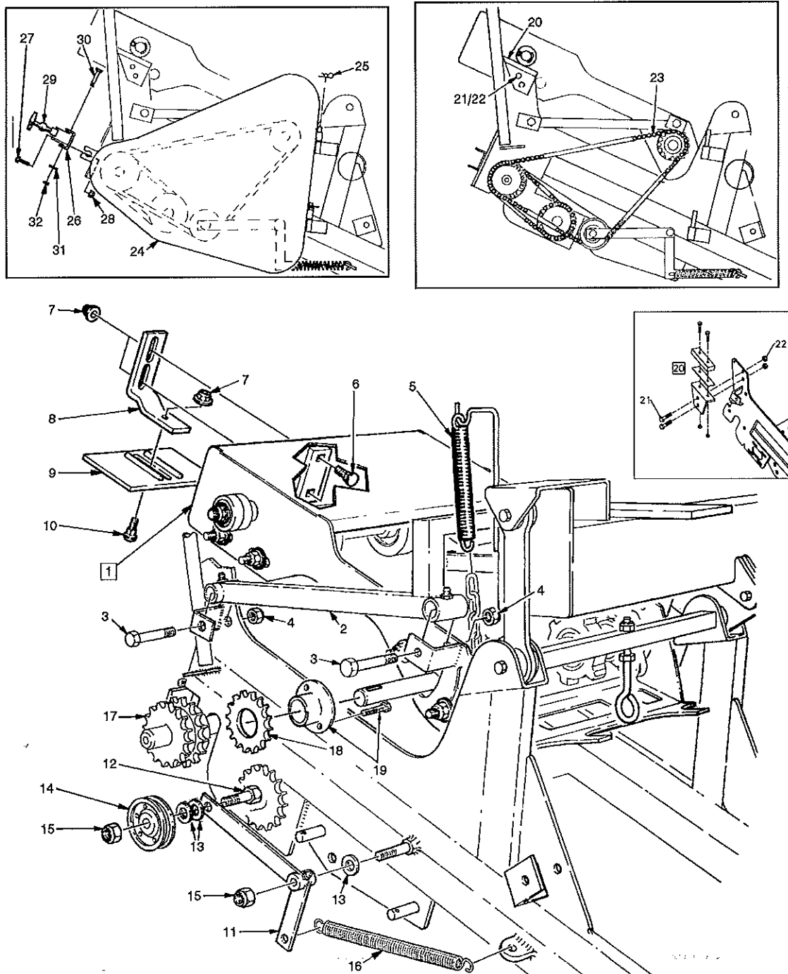
Parts List for Figure 35
