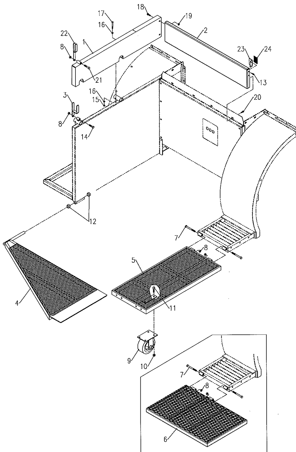
Sod Panel Extensions & Platforms Figure 55
