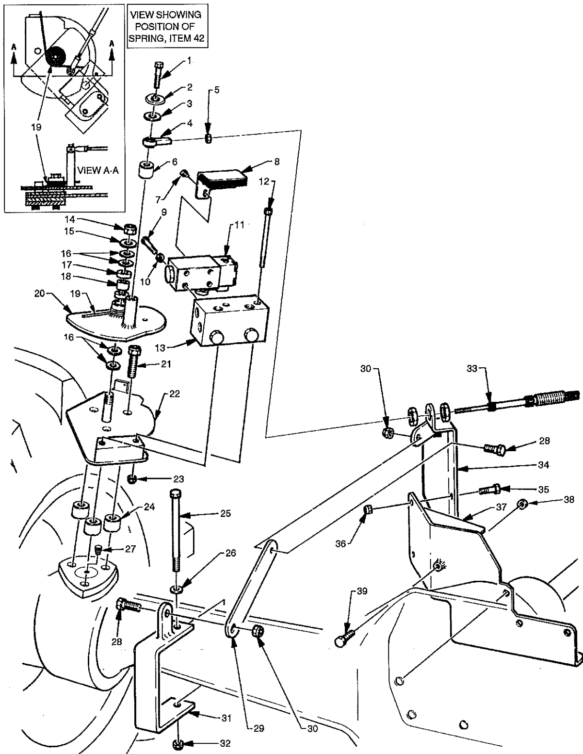
Autosteer 4 Wheel Drive Figure 48
