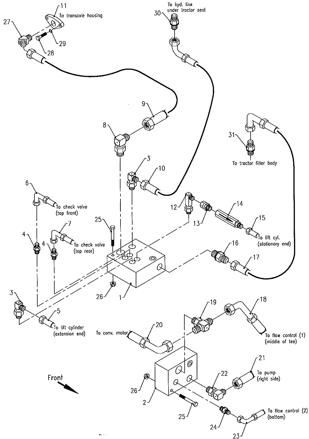
Control Valve Figure 22
