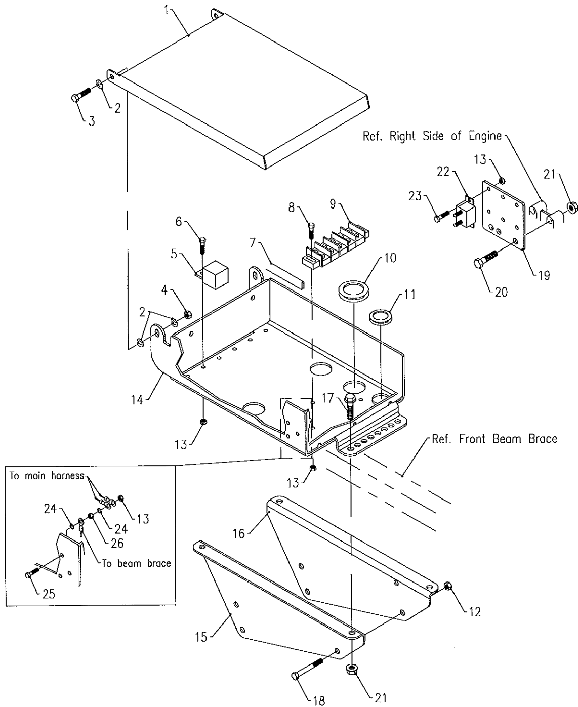
Electrical Box Breaker Mount Figure 26
