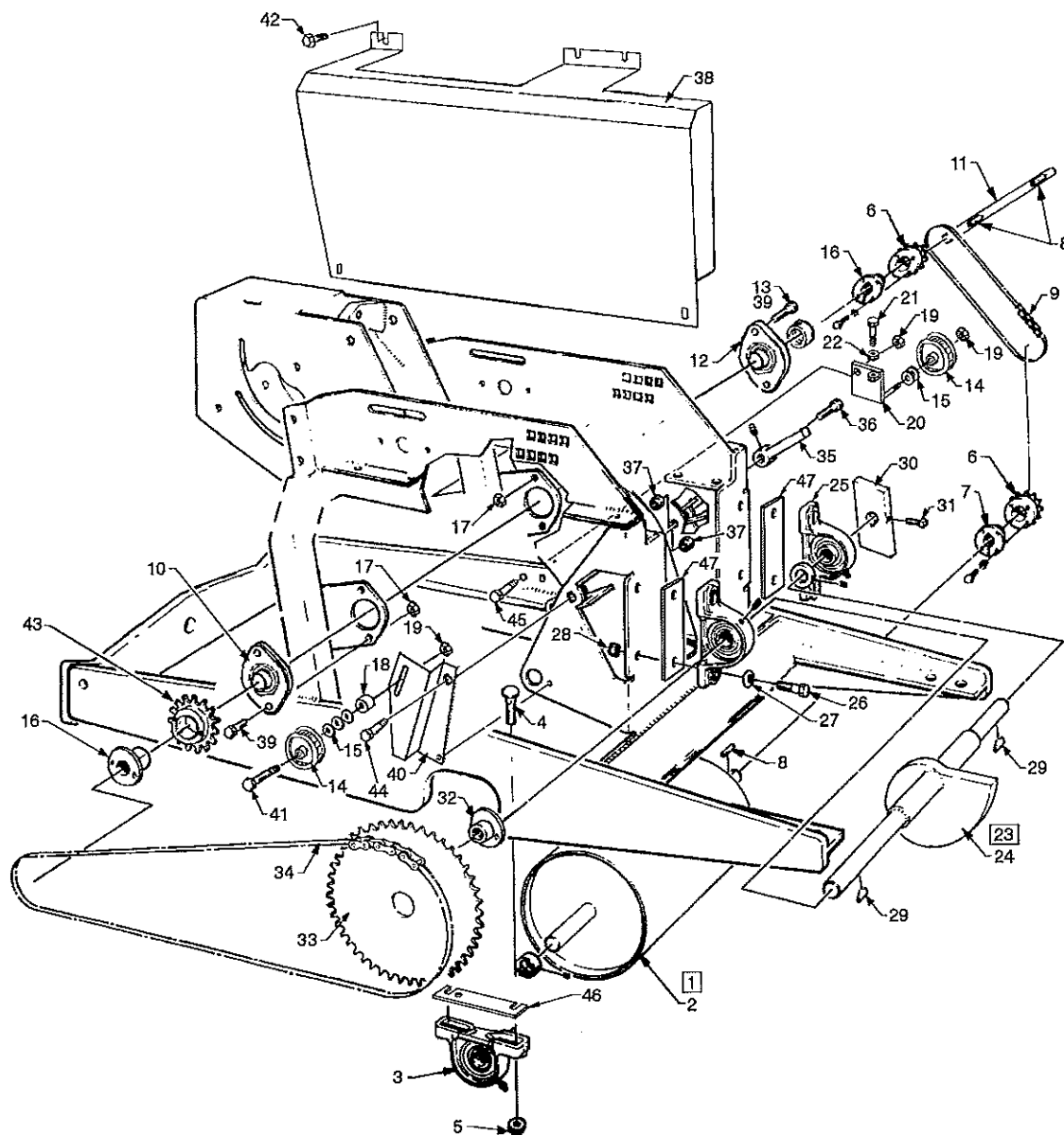
Parts List for Figure 14
