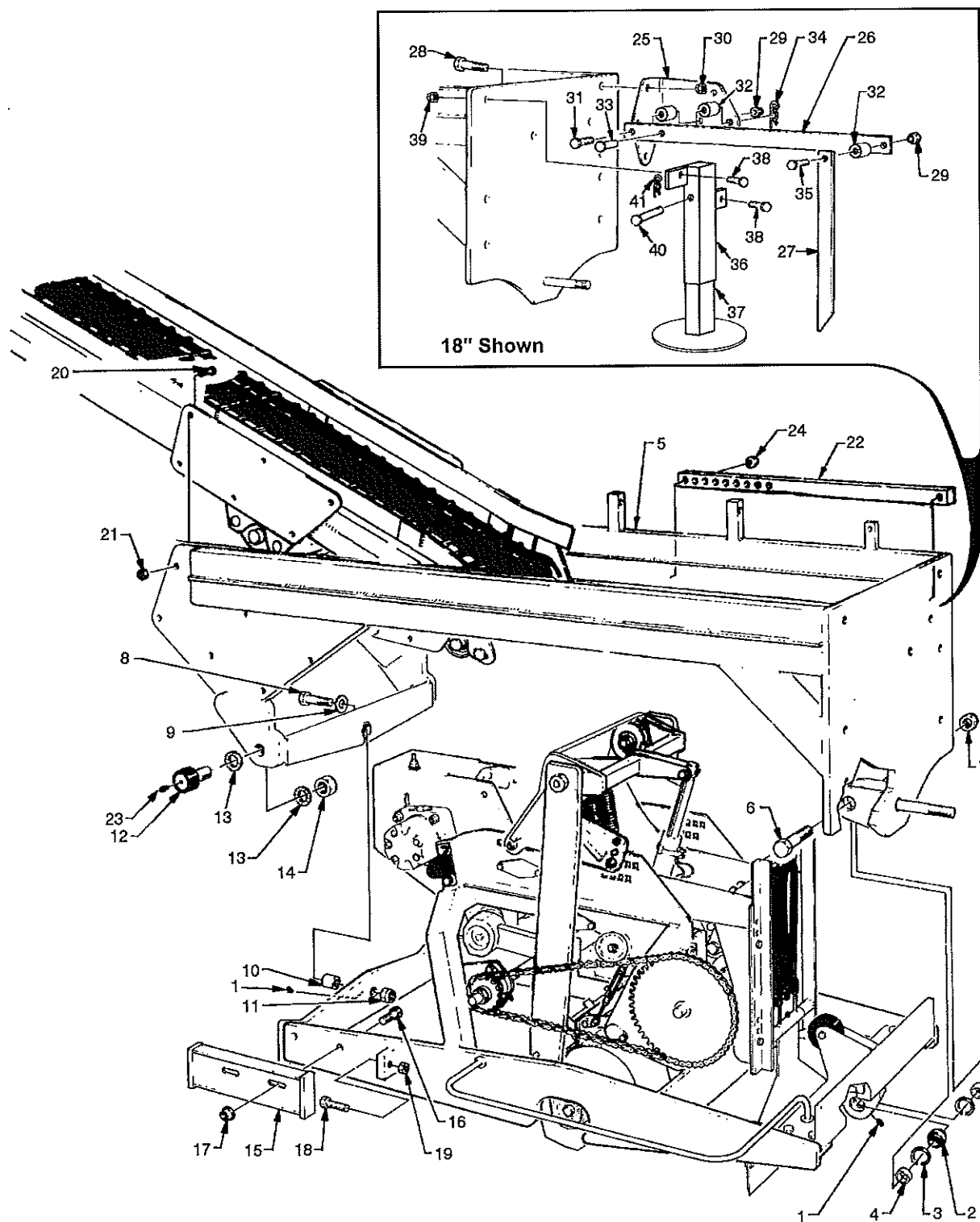
Floating Head & Cradle Figure 10
