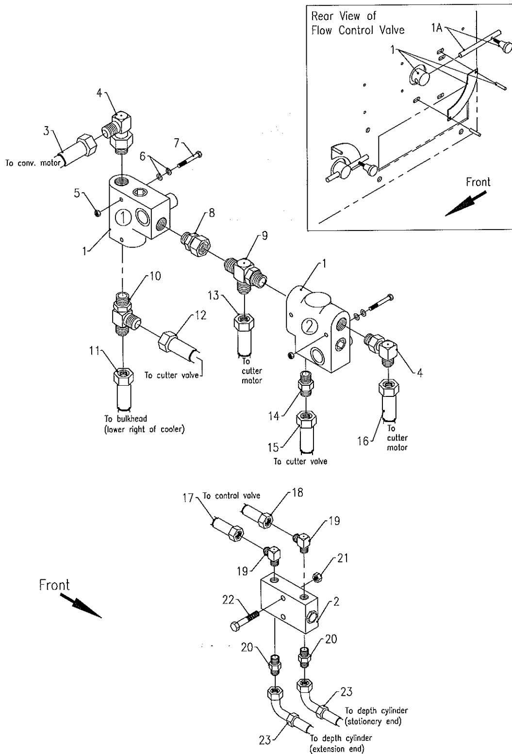
Flow Control & Check Valves Figure 23
