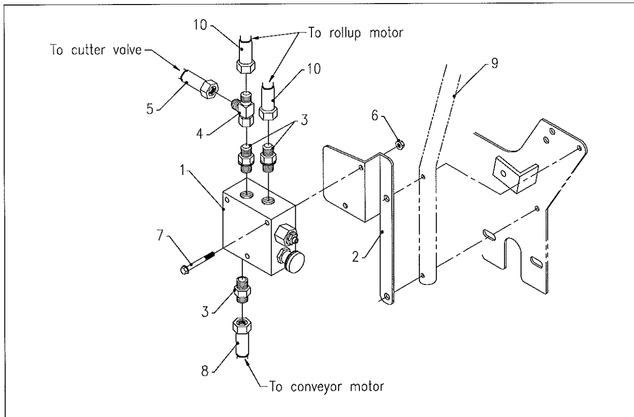
Optional Hydraulic Roll-up Figure 36
