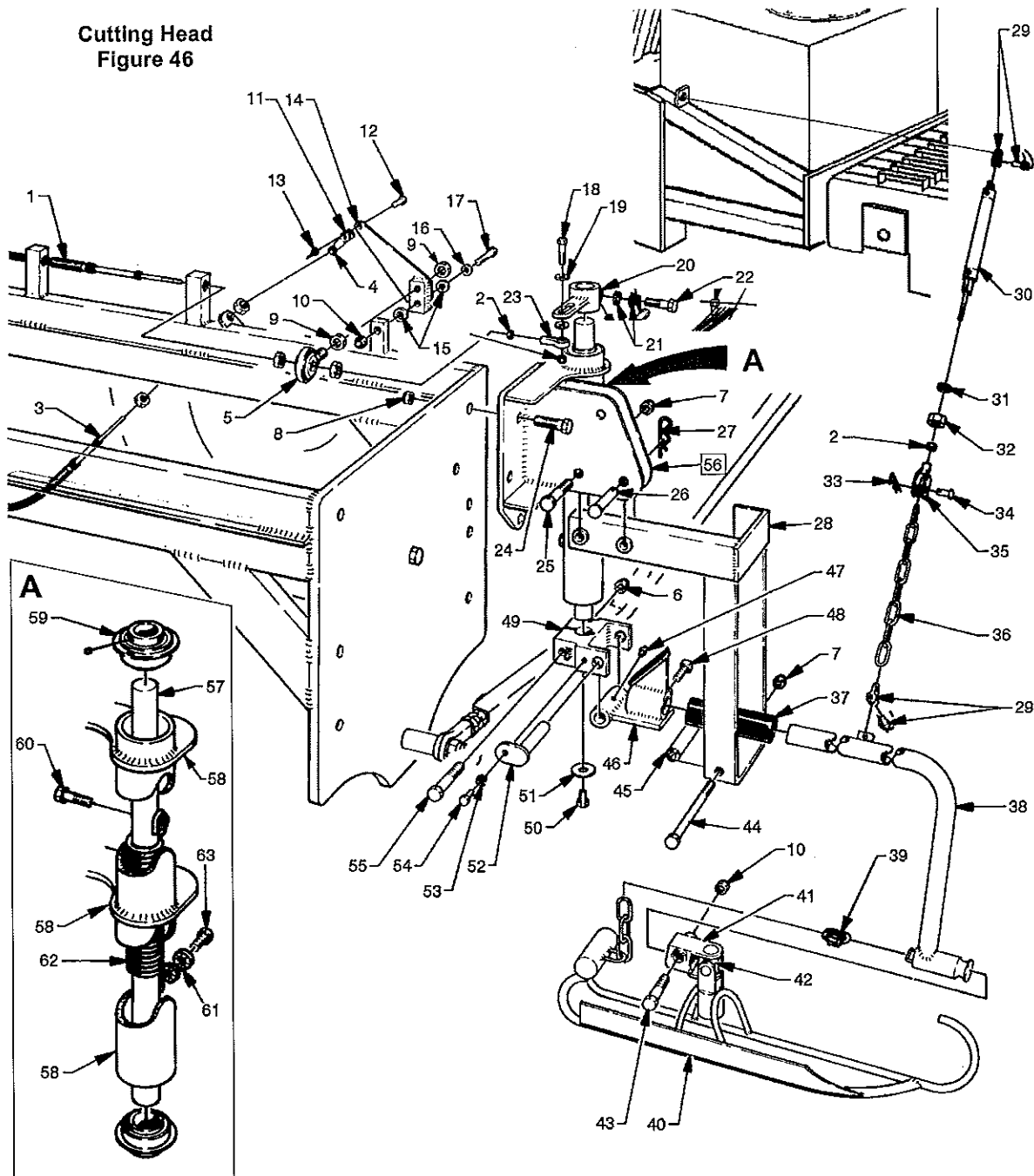
Parts List for Figure 46
