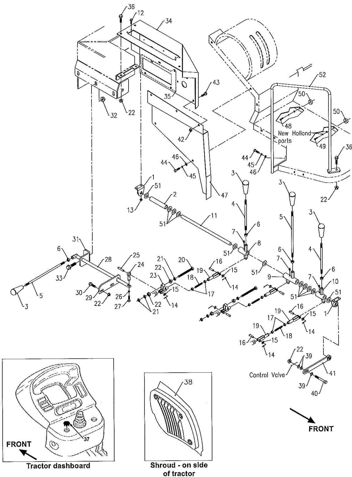
Control Panel & Linkage Figure 4
