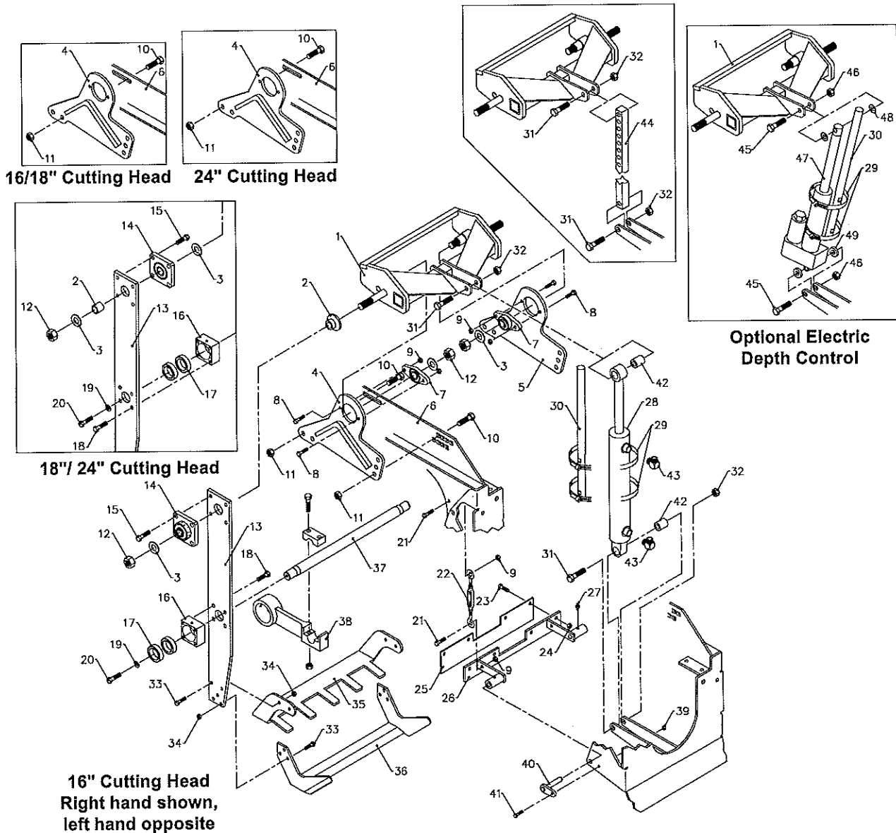
Cutting Blade Arms & Depth Control Figure 12
