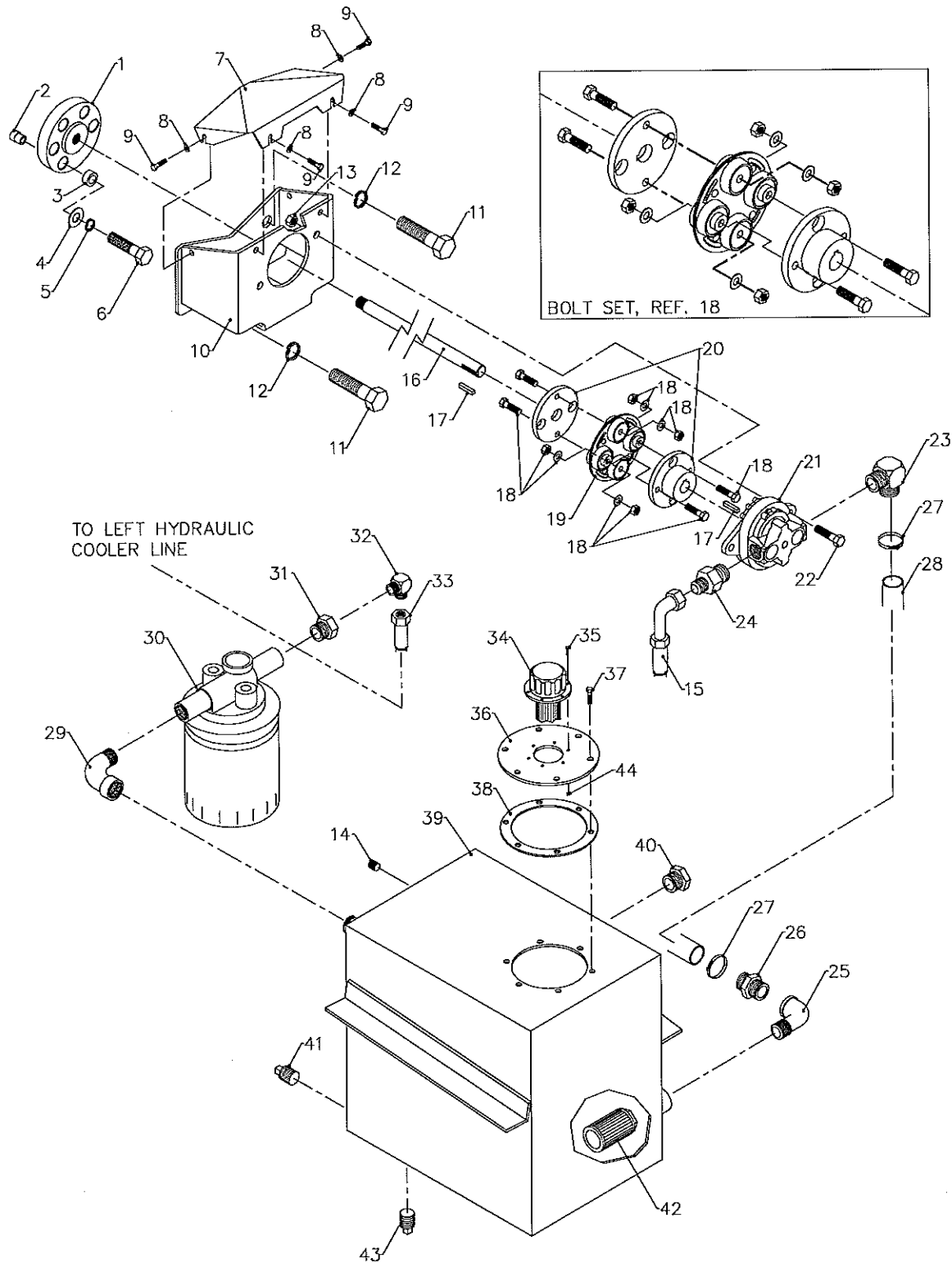
Hydraulic Tank & Pump Figure 21A
