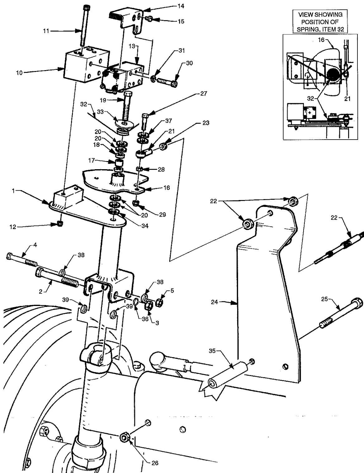
Autosteer 2 Wheel Drive Figure 47
