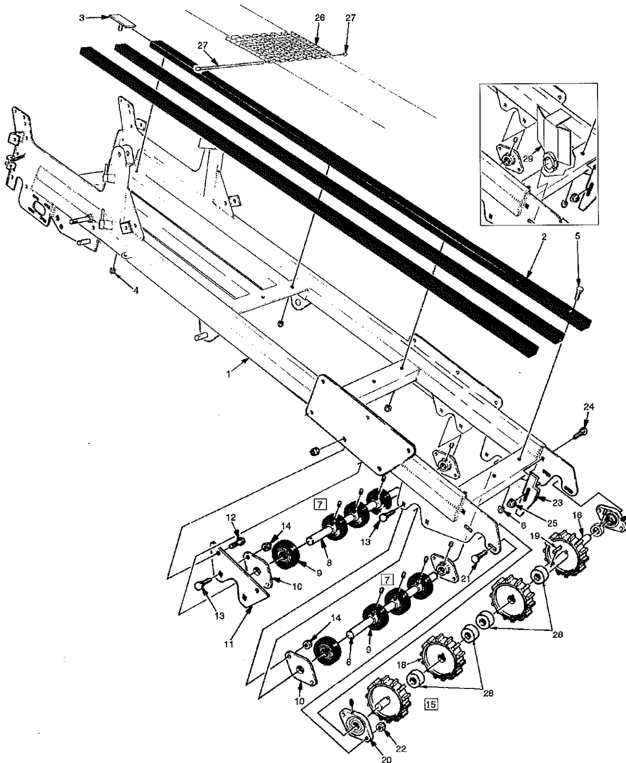
Front Idlers & Sliders Mintex Mat, 24" Figure 17
