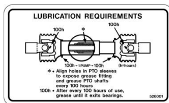
ITEM 9 (526001)
