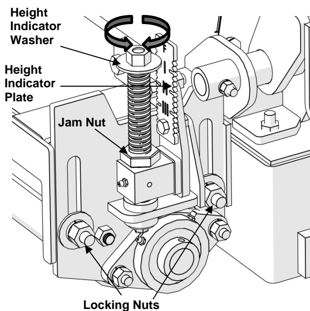
HEIGHT ADJUSTER BETWEEN WING DECKS (8) PLACES
