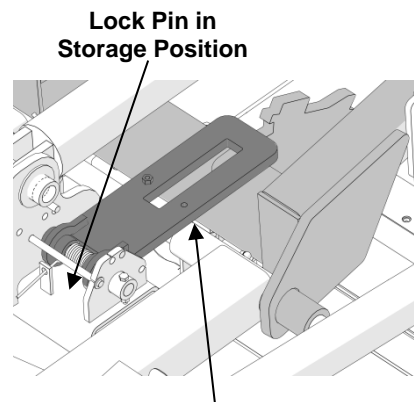
Lock plate flat on wing plate
