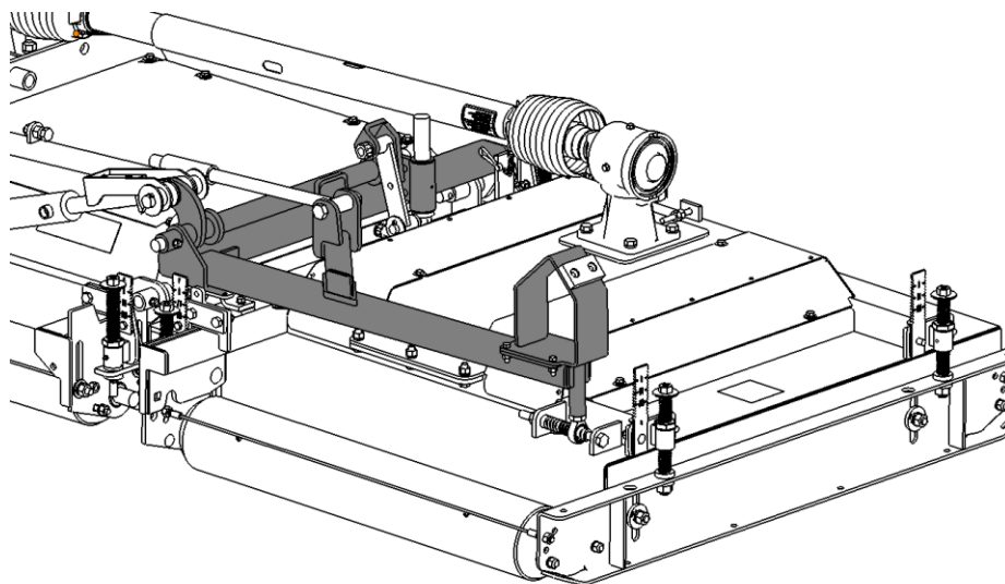
Outer Wing Deck Installed onto Main Wing Deck
