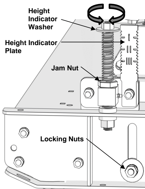
HEIGHT ADJUSTER ON OUTER ENDS OF DECKS (12) PLACES
