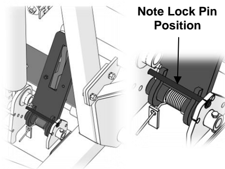
TRANSPORT LOCK POSITION - WINGS
