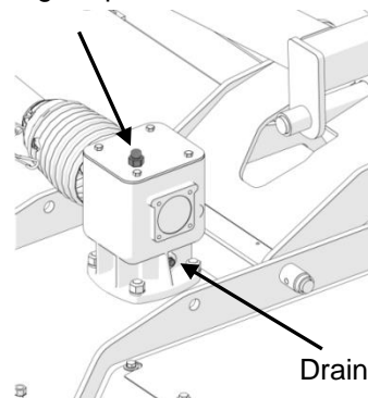
Fill Plug / Dipstick
