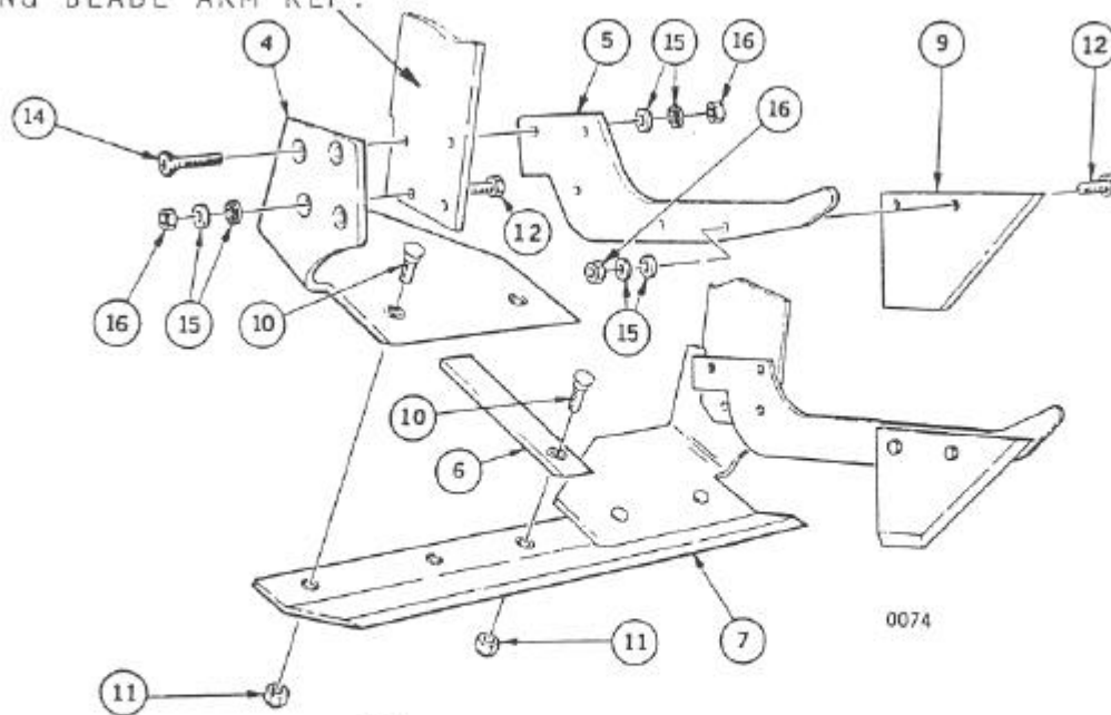
2 3 PIECE UNIBLADE, 18"
