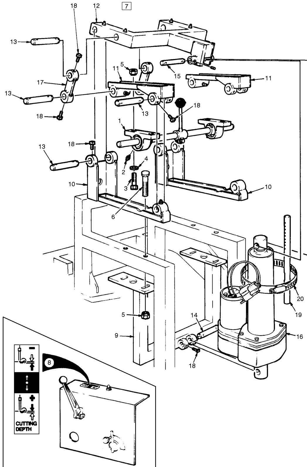
Electric Depth Control Assembly Figure 33-1
