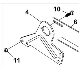
24" CUTTING HEAD
